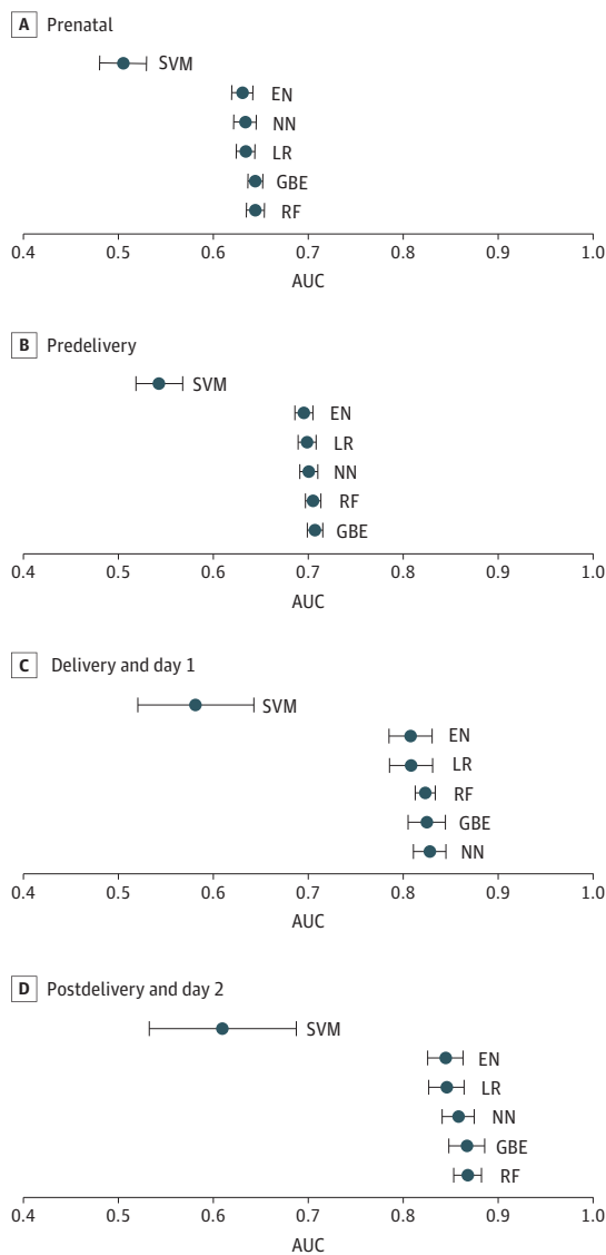
Figure 2. Mean (95% CI) for Validation AUC by Scenario for Outcomes of Intrapartum Stillbirth and Neonatal Mortality
