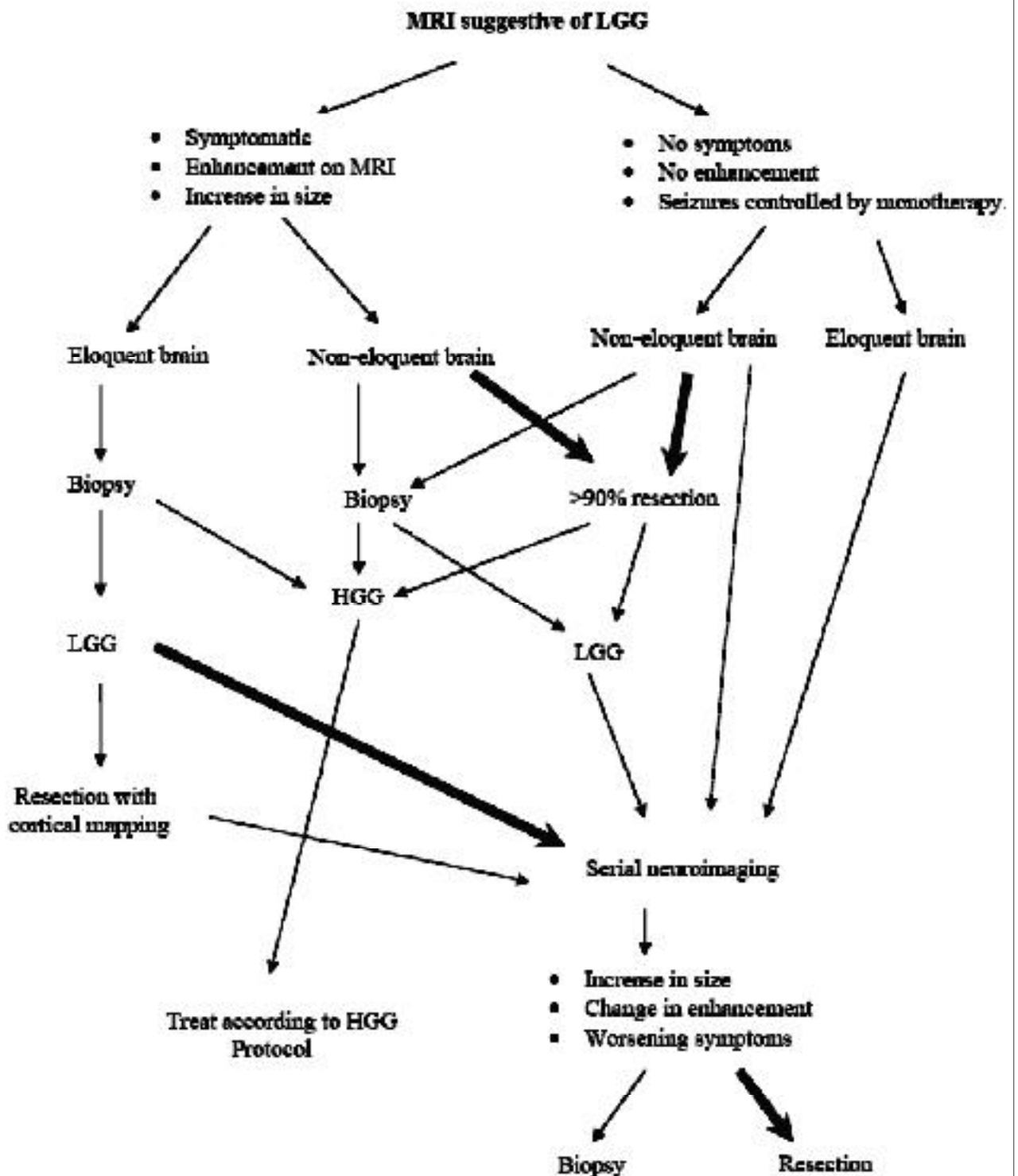
Figure 8. Decision-making in LGG. At junctures where multiple options are available, the preferred option is marked by a thicker arrow.
